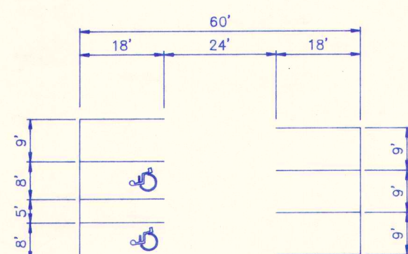
TYPICAL PARKING DETAIL 1" = 20'
