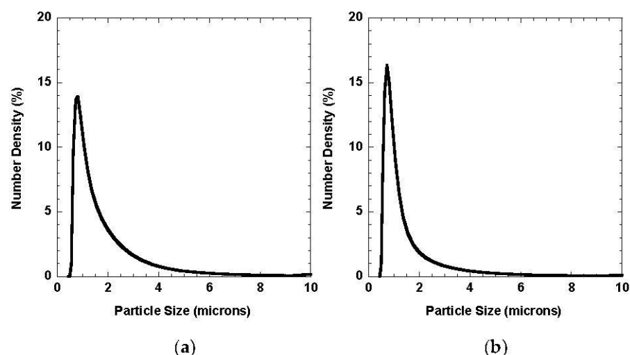
Figure 2. Fits to laser diffraction measurements of (a) cement and (b) concrete dust.
