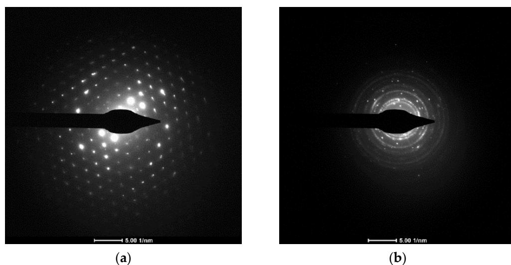
Figure 5. SAED pattern of (a) cement and (b) concrete dust.
