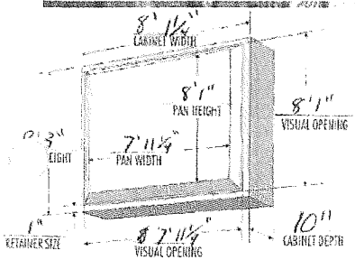
Existing Elevation
