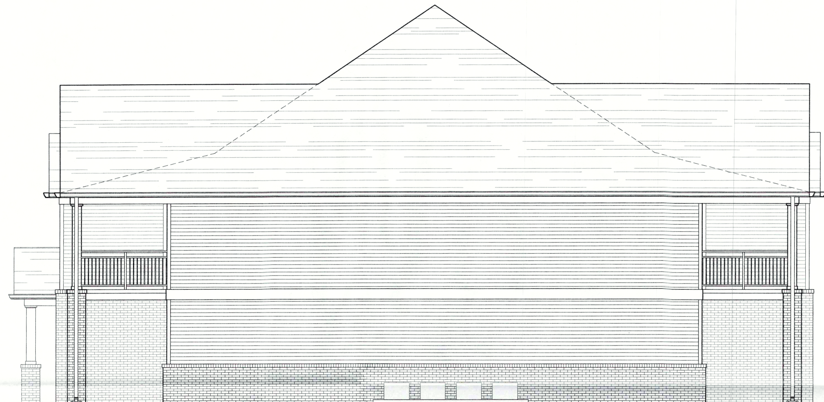
BUILDING TYPE A1 (16-PLEX) RIGHT SIDE ELEVATION
