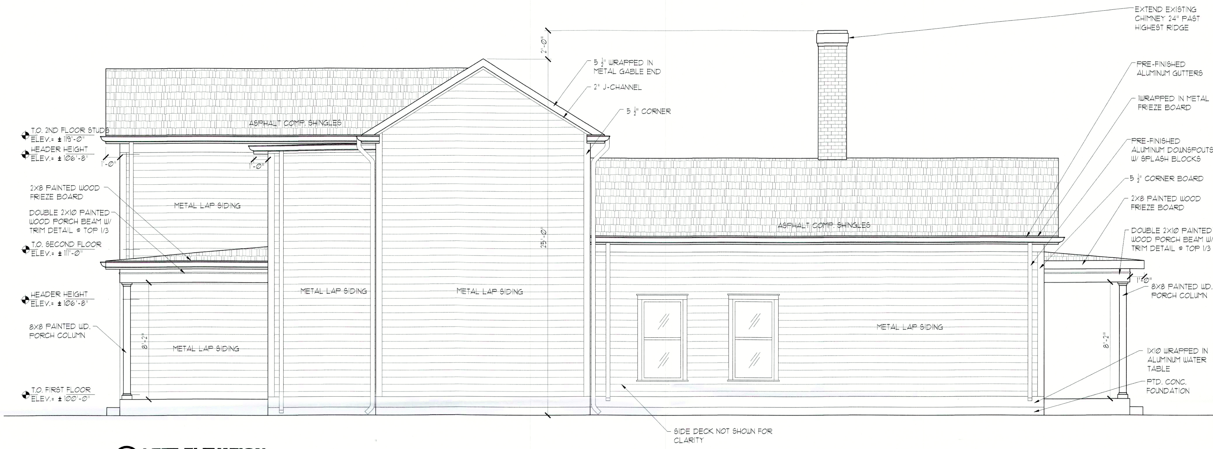
2 LEFT ELEVATION SCALE 1/4"=1'-0"
