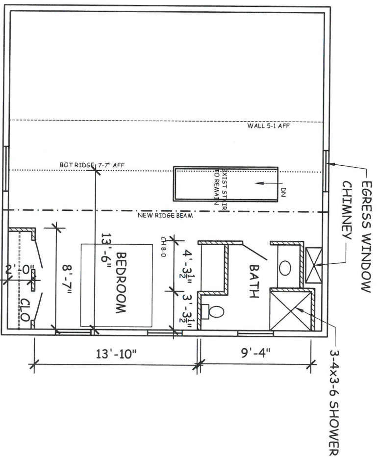
ATTIC PLAN 1/8"=1'-0"
