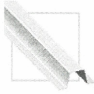
ROOF PURLINS 18 Gauge Galvanized Roof Purlins 4' 9 3/4" On Center Spacing
