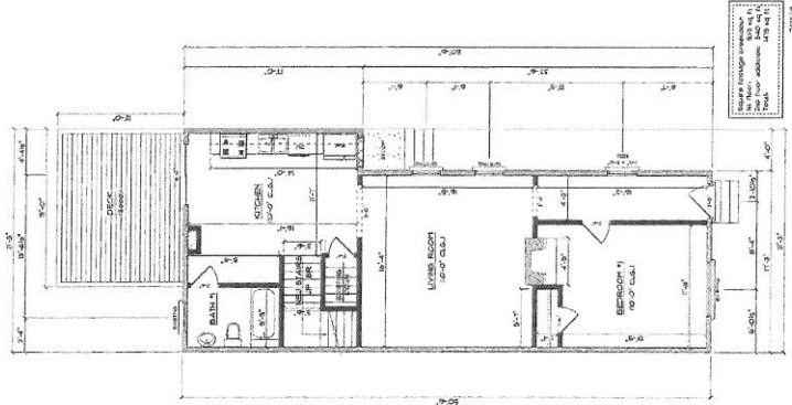
PROPOSED 1ST FLOOR (B)
