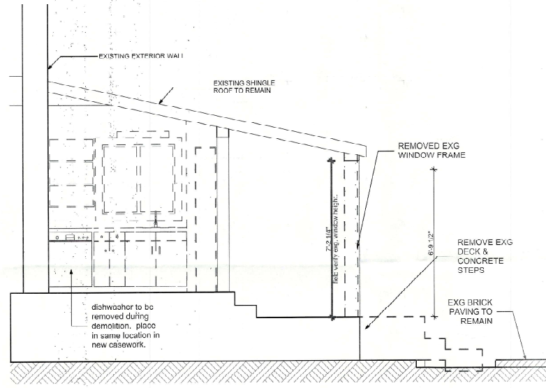
2 BUILDING SECTION SCALE: 1/4" = 1'-0"
