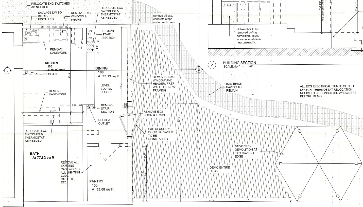
1 EXISTING & DEMO PLAN SCALE: 1/4" = 1'-0"
