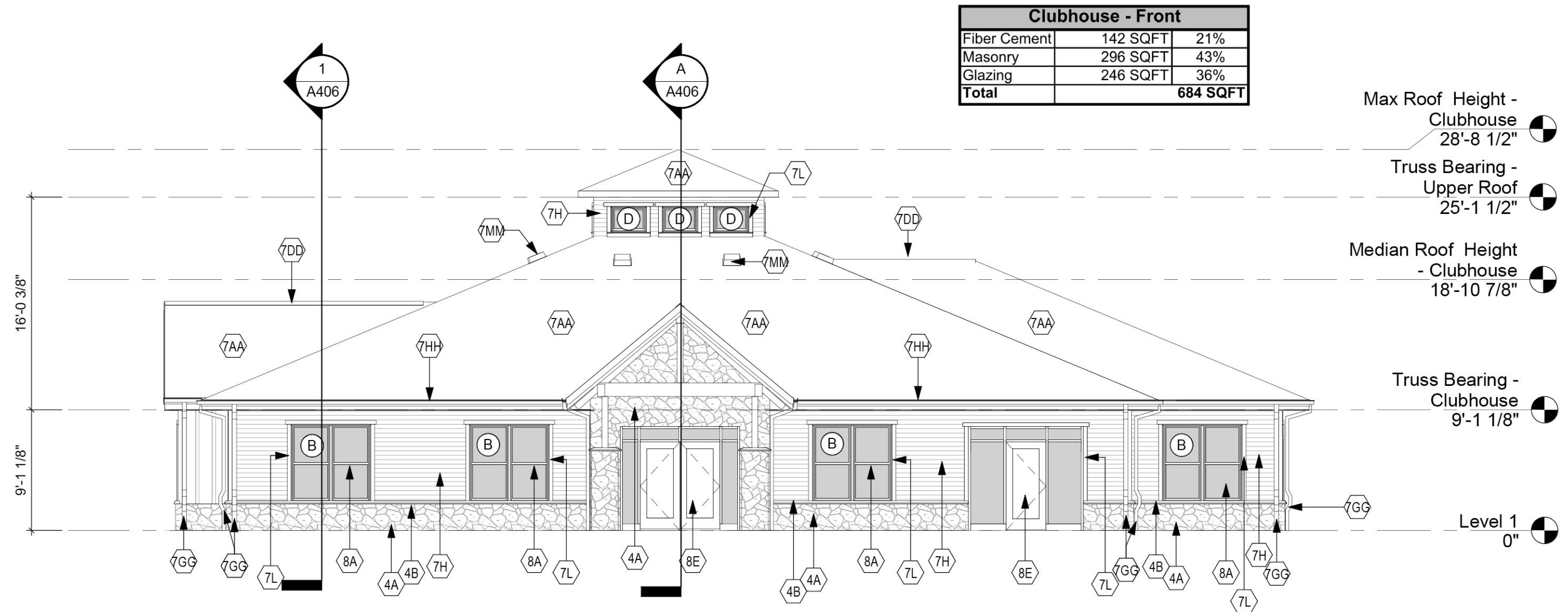
1 Elevation - Clubhouse - Front A211 1/8" = 1'-0"
