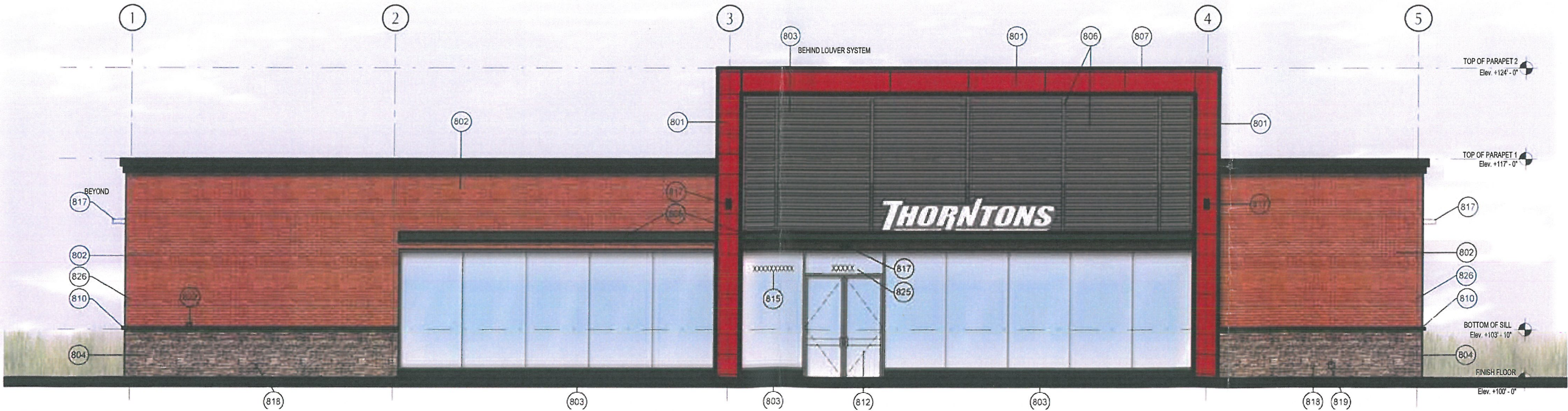
Building - Front Elevation
