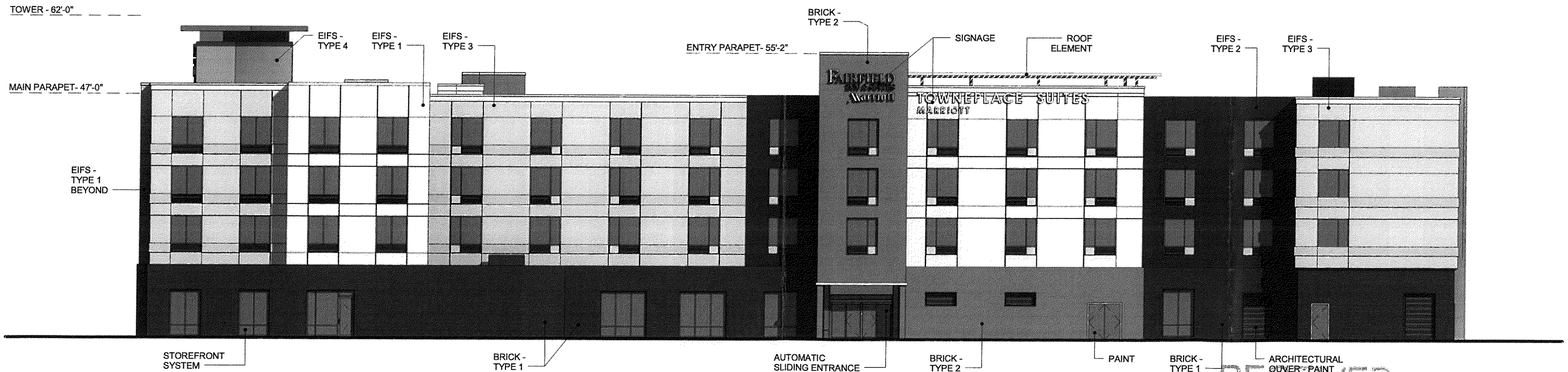
NORTH ELEVATION
