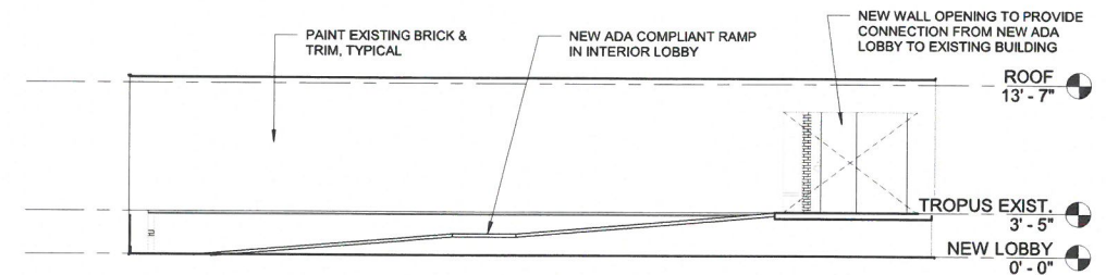
3 INTERIOR LOBBY ELEVATION - TROPUS BUILDING 1/8" = 1'-0"
