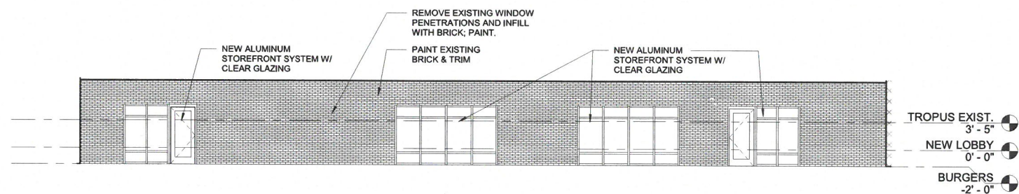
2 INTERIOR ATRIUM ELEVATION - BURGER'S MARKET 1/8" = 1'-0"
