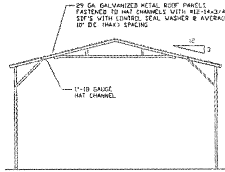
TYPICAL SECTION VERTICAL ROOF OPTION SCALE: NTS
