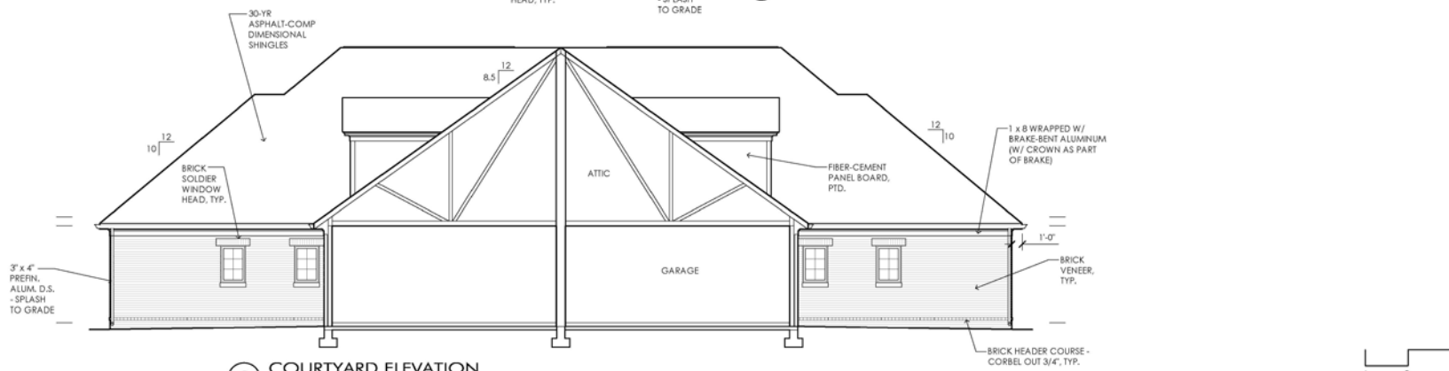
3 COURTYARD ELEVATION
