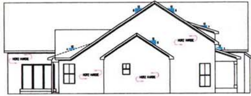
LEFT ELEVATION 1/8" = 10'
