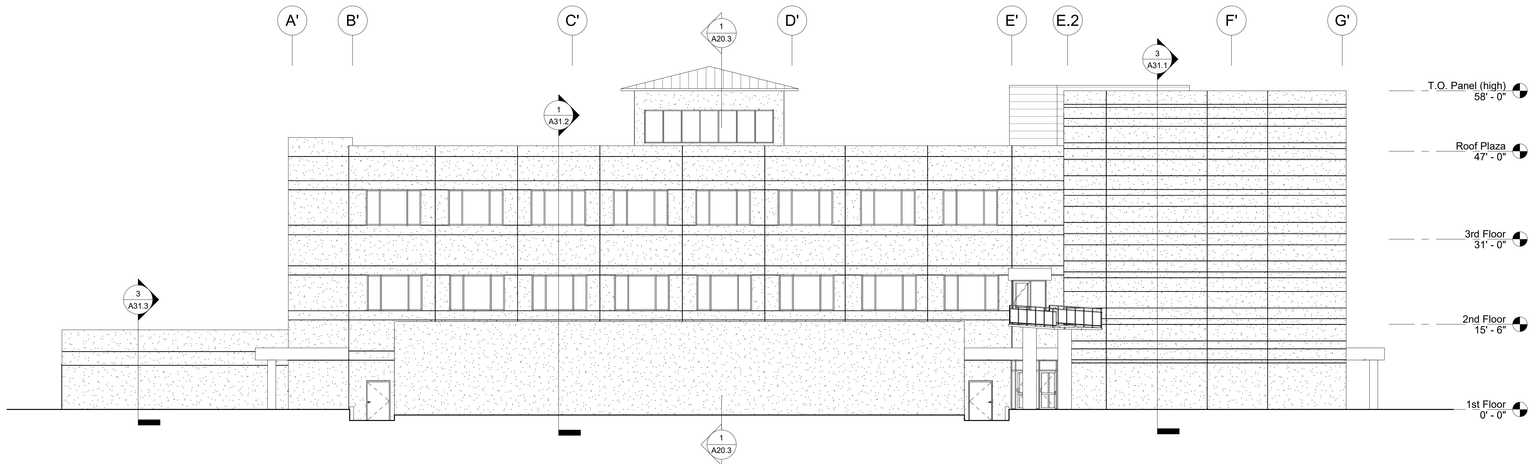
4 North Elevation 3/32" = 1'-0"
