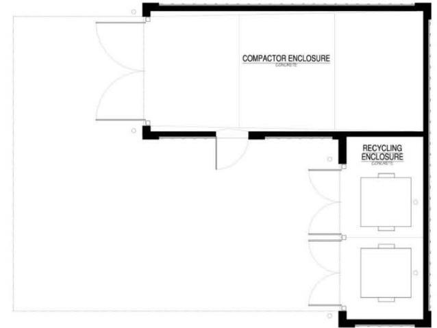
Compactor/Recycling Enclosure Floor Plan SCALE: 1/8"=1'-0"
