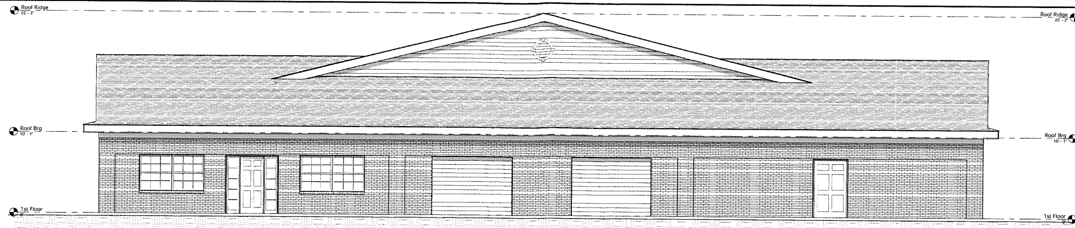
4 Right Elevation 3/16" = 1'-0"
