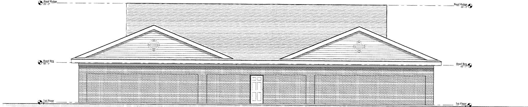
3 Rear Elevation 3/16" = 1'-0"
