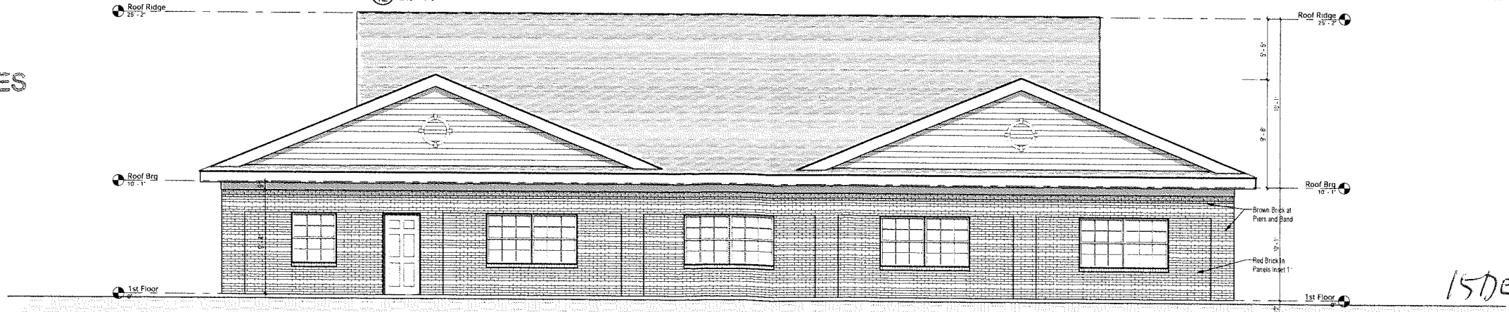
1 Front Elevation (Old Bardstown Rd.) 3/16" = 1'-0"
