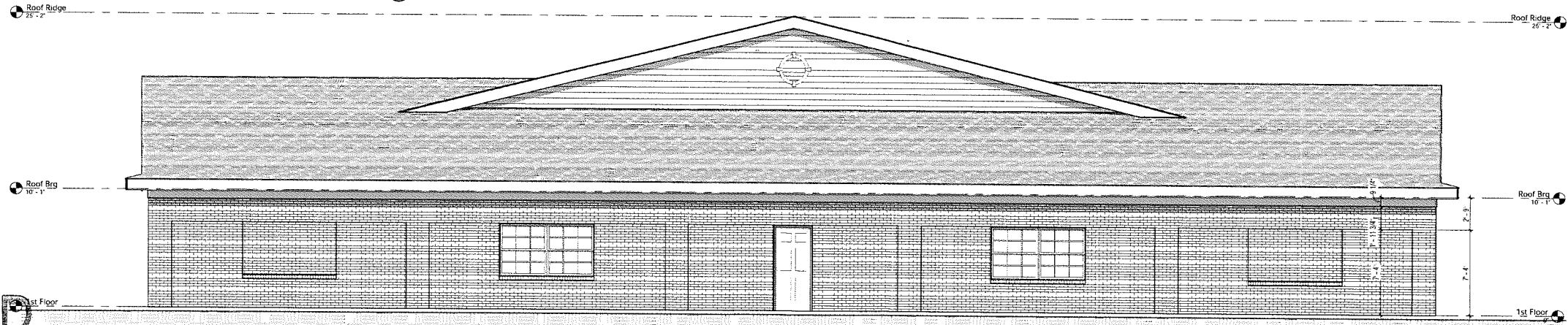
2 Left Elevation 3/16" = 1'-0"
