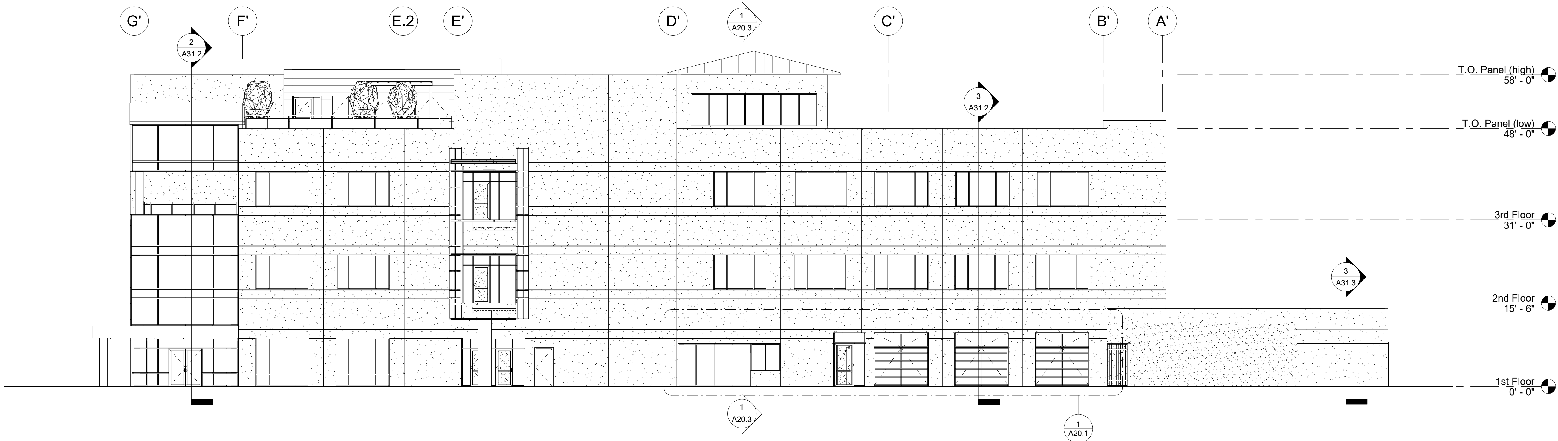
3 South Elevation 3/32" = 1'-0"
