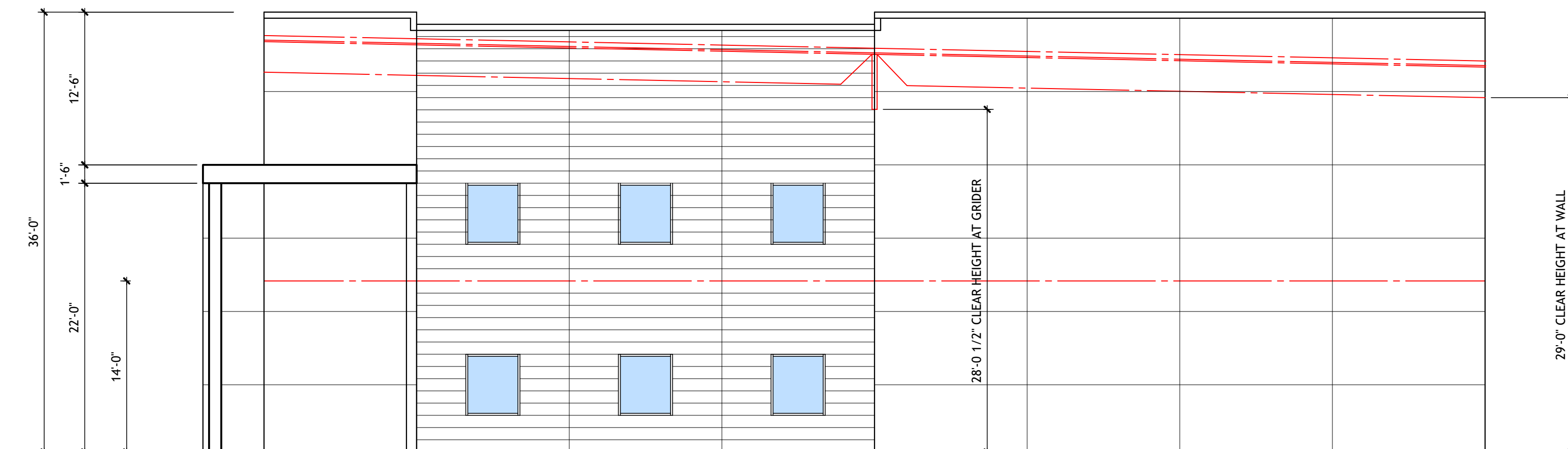
2 A-501 South (Right) Elevation full size plot scale: 1/8"=1'-0" 0 4'-0" 8'-0"
