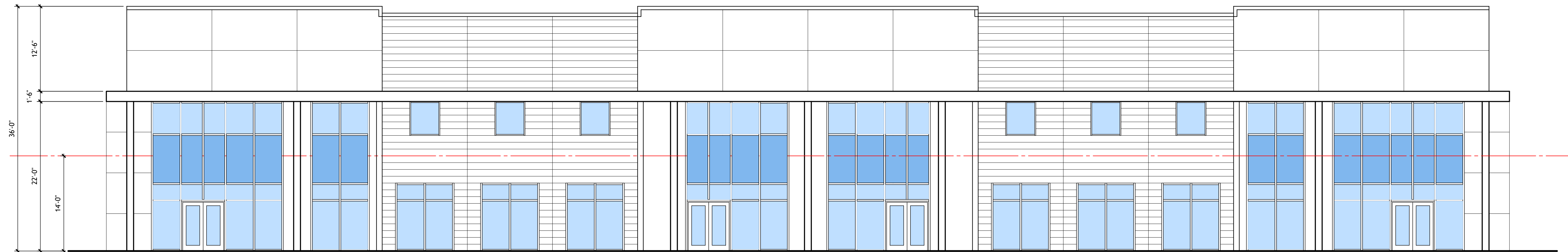
1 A-501 West (Front) Elevation full size plot scale: 1/8"=1'-0" 0 4'-0" 8'-0"
