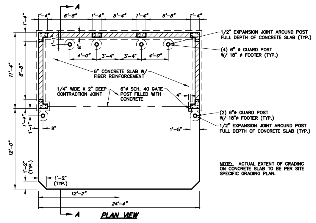
CMU DUMPSTER ENCLOSURE NO SCALE
