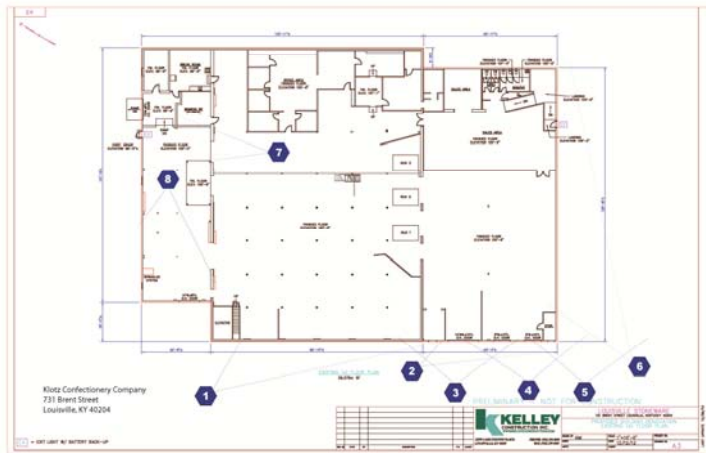
First-floor Plan
