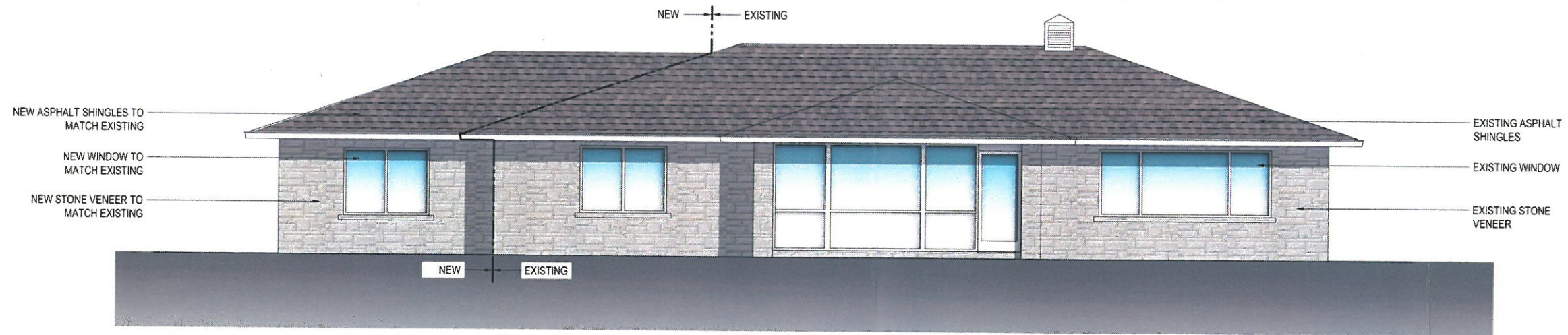
FRONT ELEVATION Scale: 1/4" = 1'-0"
