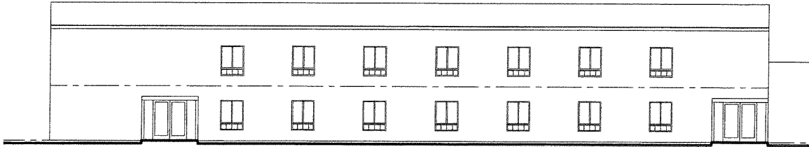
Revovated West Elevation 1/8"=1'-0"
