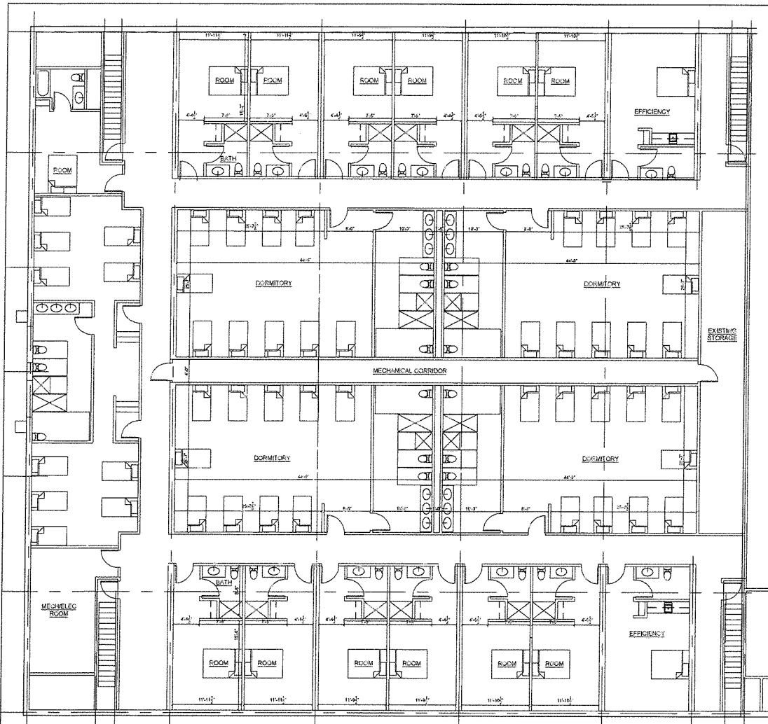
2nd Floor Schematic Plan 1/8"=1'-0"
