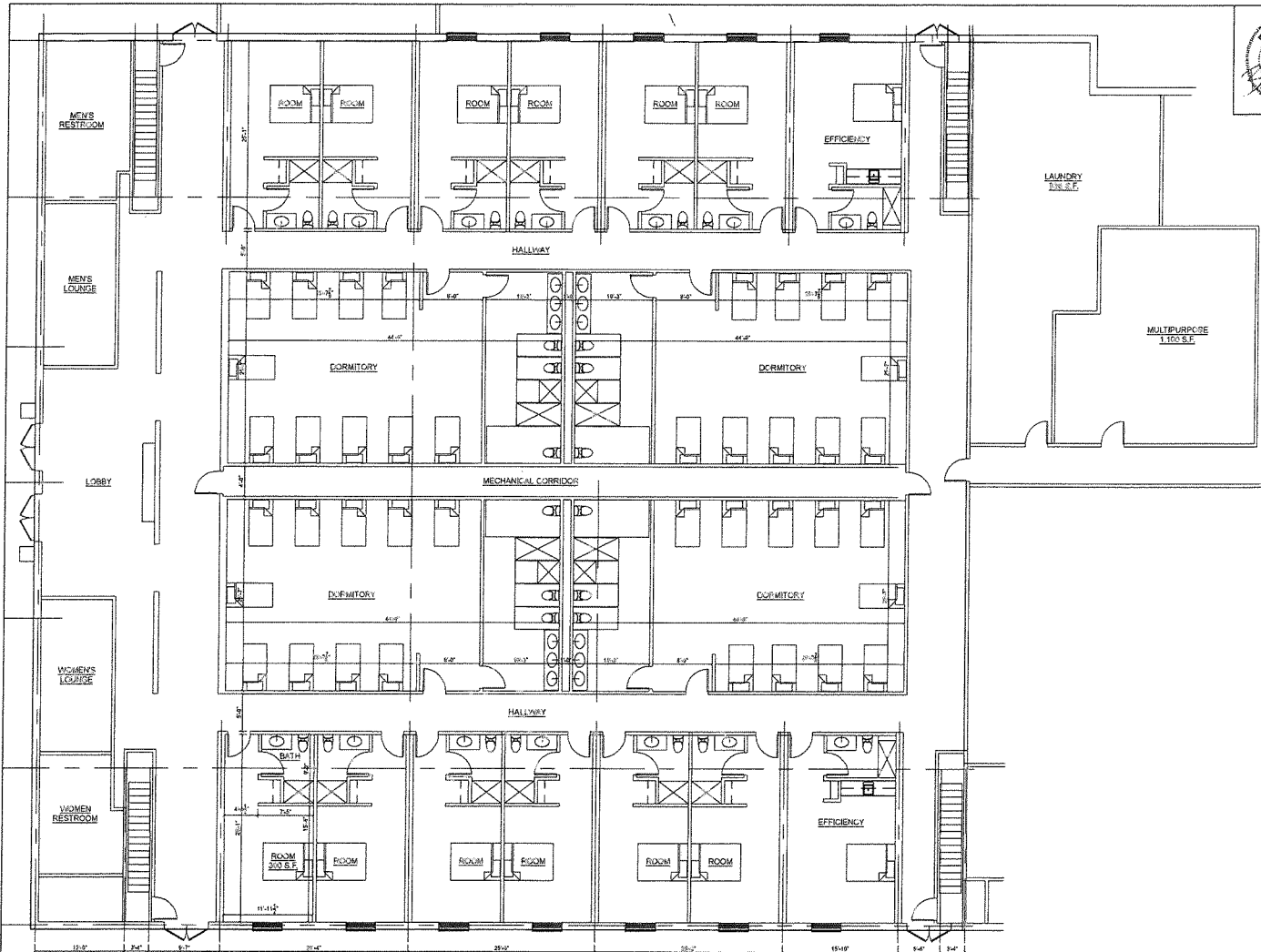
1st Floor Schematic Plan 1/8"=1'-0"
