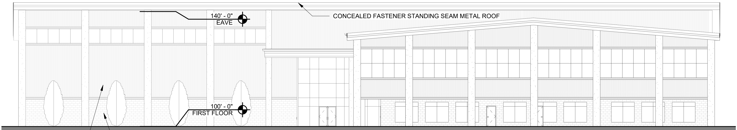
1 CHAMBERLAIN LN. STREET SIDE 1/16" = 1'-0"
