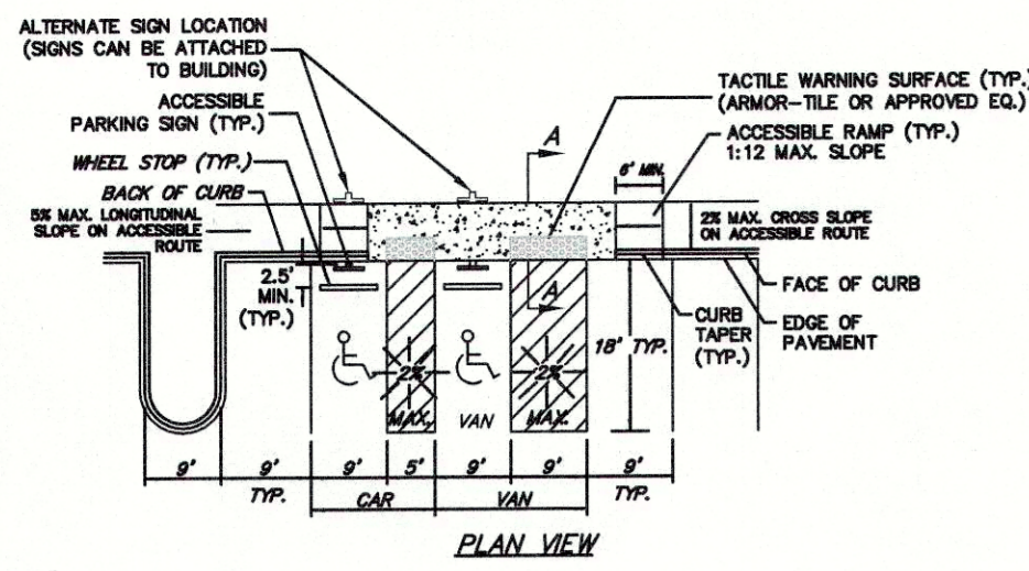
TYPICAL ACCESSIBLE PARKING SPACES NO SCALE
