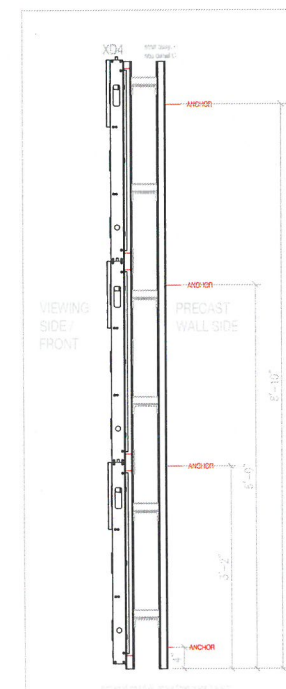
D. Side View, typical of 8 assemblies
