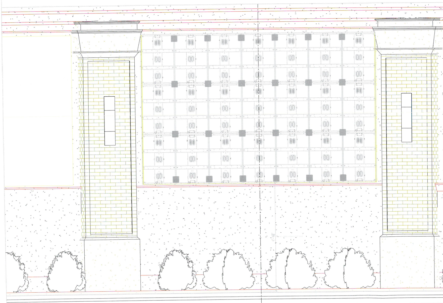
B. Strut Attachment, elevation / projection
