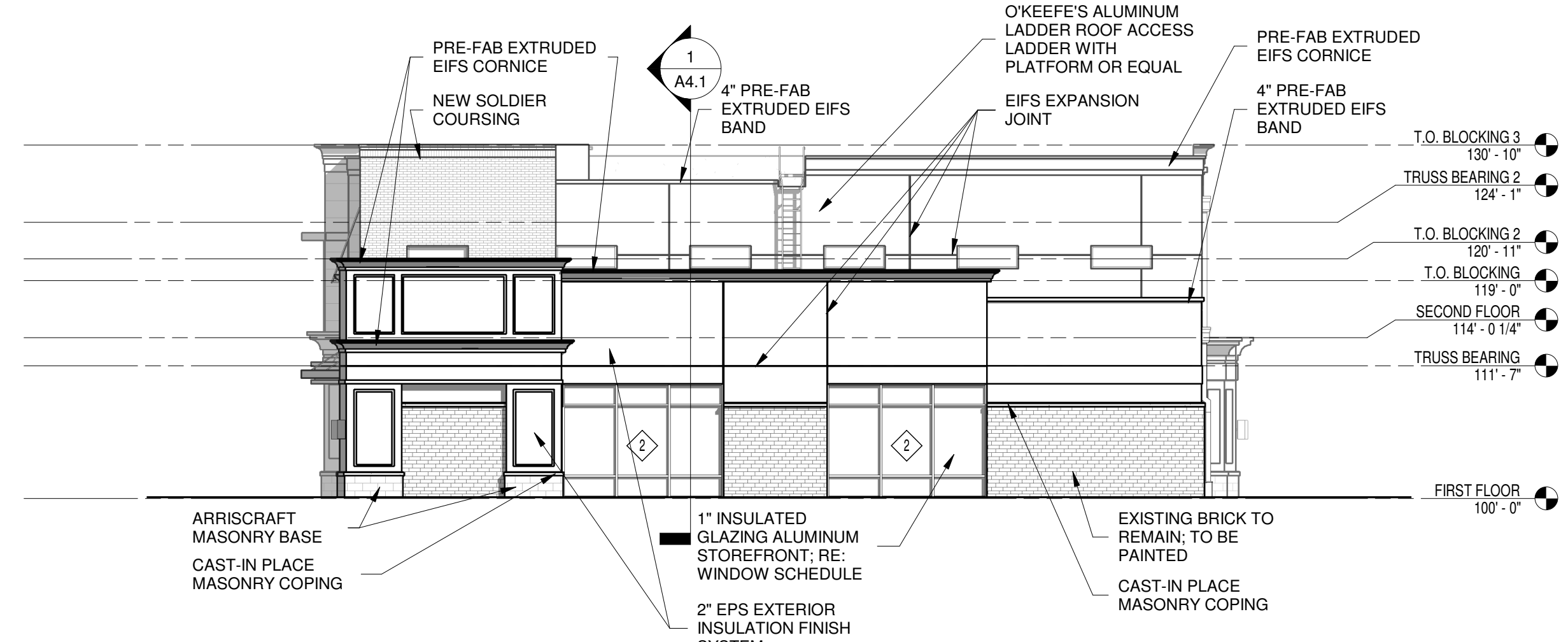
4 Overall Elevation East 3/32" = 1'-0"
