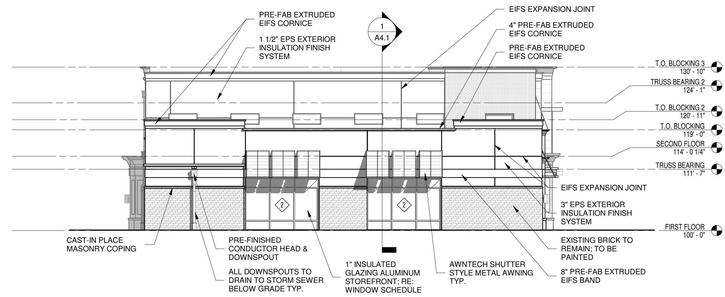
3 Overall Elevation West 3/32" = 1'-0"
