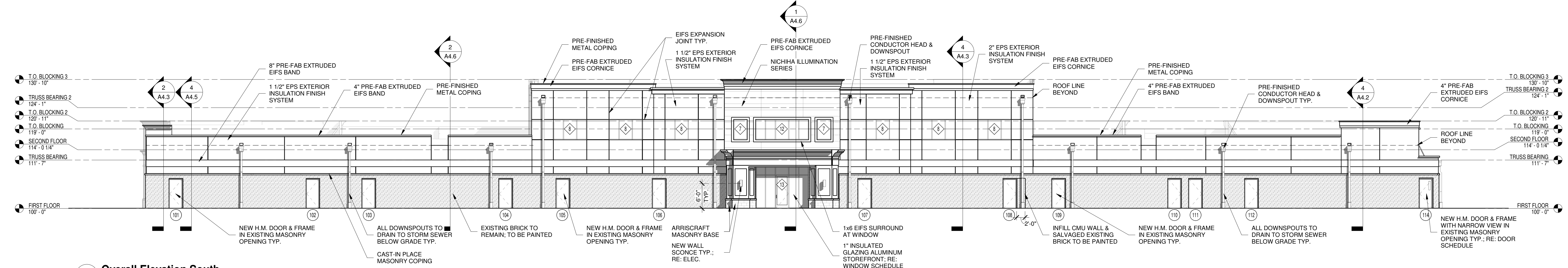
2 Overall Elevation South 3/32" = 1'-0"
