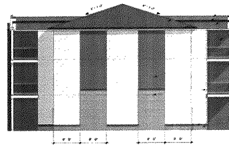
2 bdrm - west elevation
