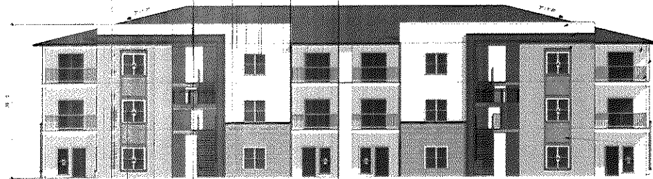
Type B - south elevation
