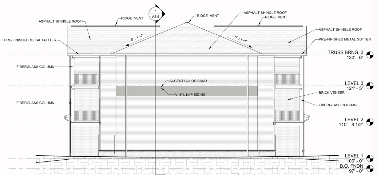
2 BUILDING ELEVATION 1/8" = 1'-0"
