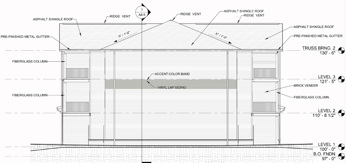
2 BUILDING ELEVATION 1/8" = 1'-0"
