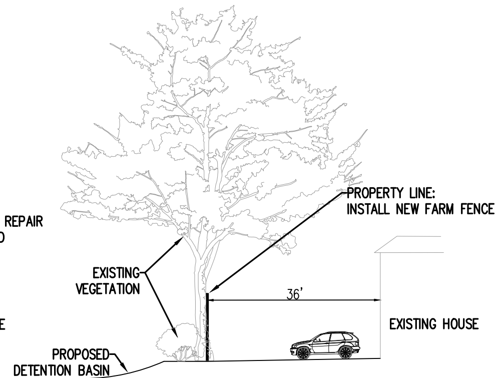
Section C-C
