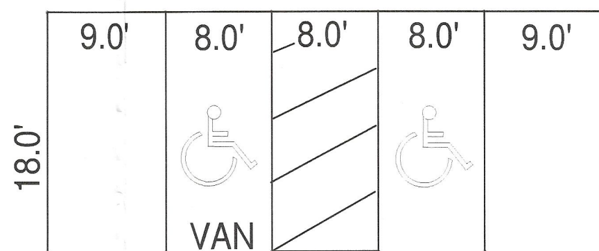
TYPICAL PARKING SPACE LAYOUT (No Scale)
