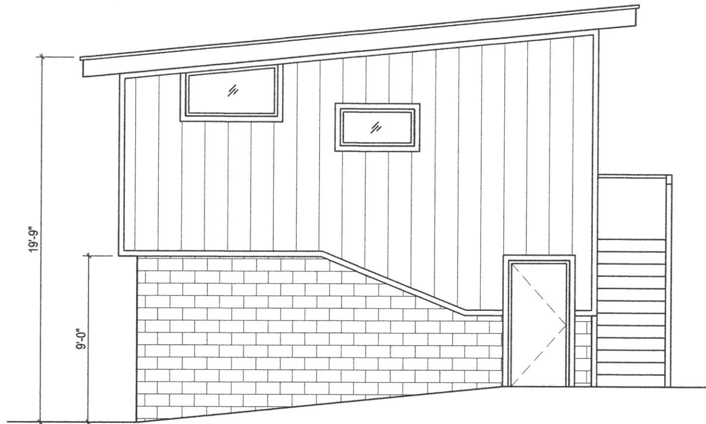
2 EAST (1618) ELEVATION SCALE: 3/16" = 1'-0"
