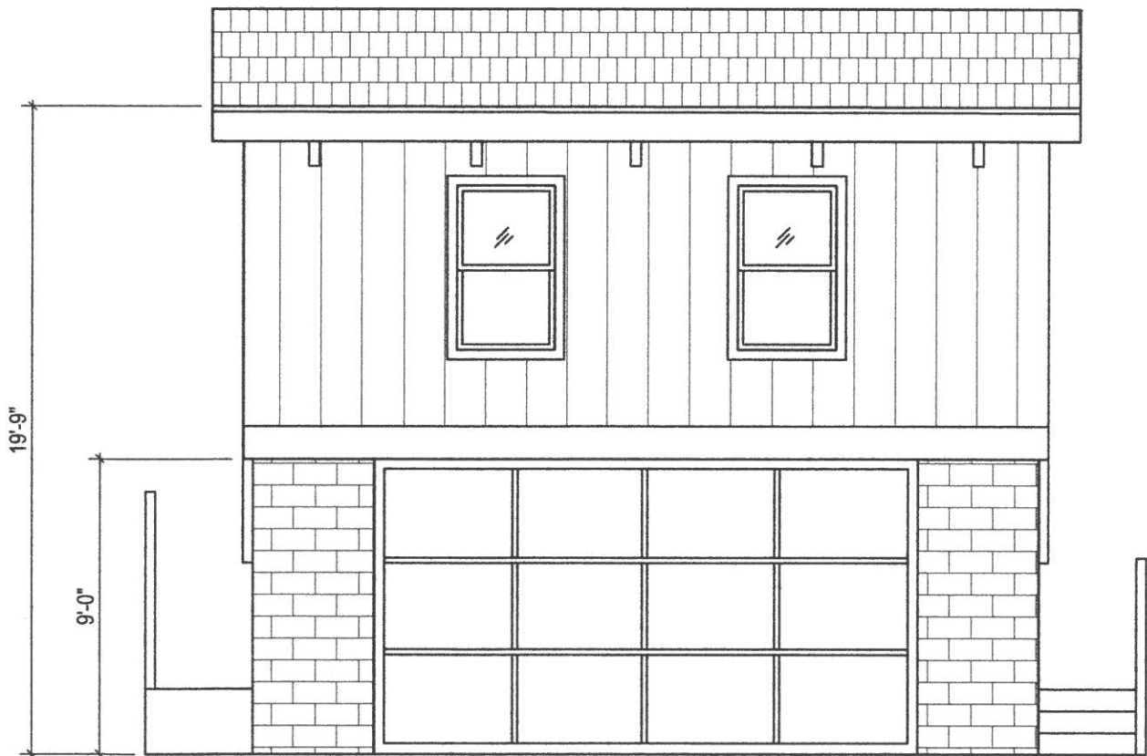
3 ALLEY ELEVATION SCALE: 3/16" = 1'-0"
