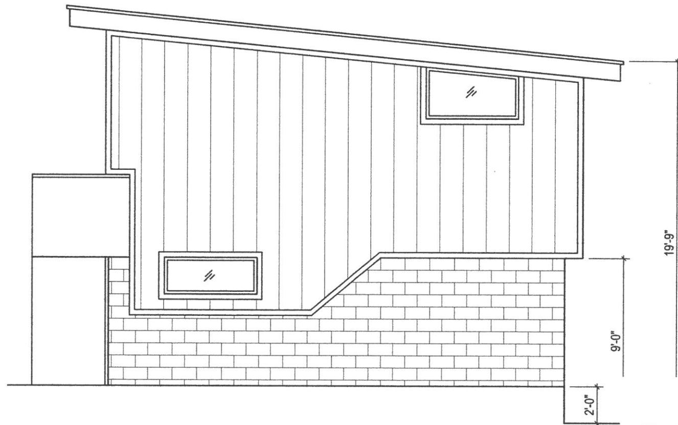
4 WEST (1614) ELEVATION SCALE: 3/16" = 1'-0"
