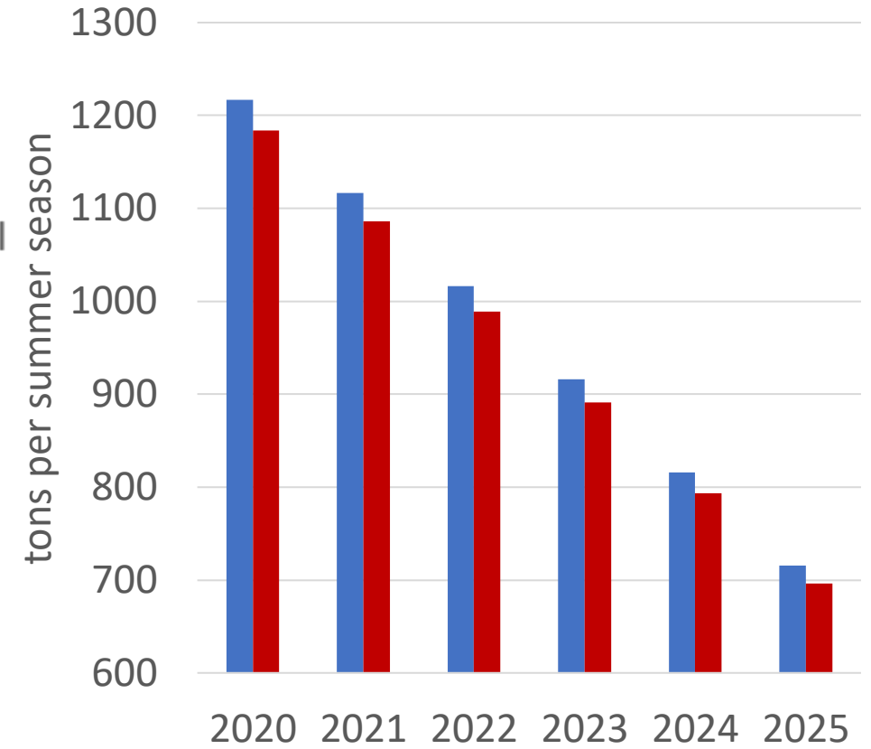
NOx Emissions
