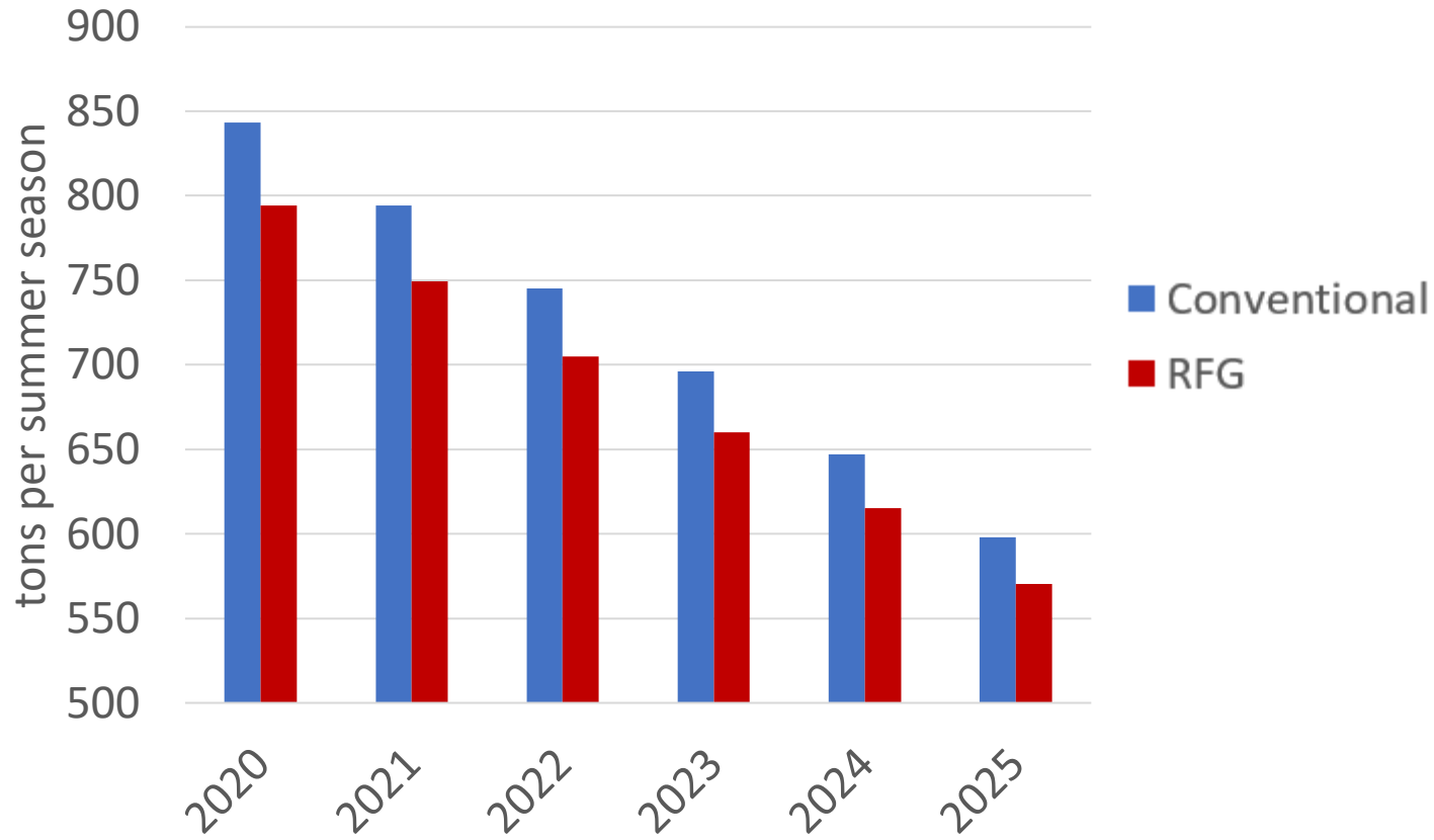
VOC Emissions
