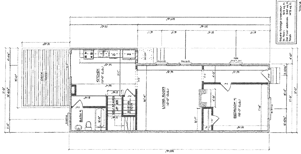
PROPOSED 1ST FLOOR (B)
