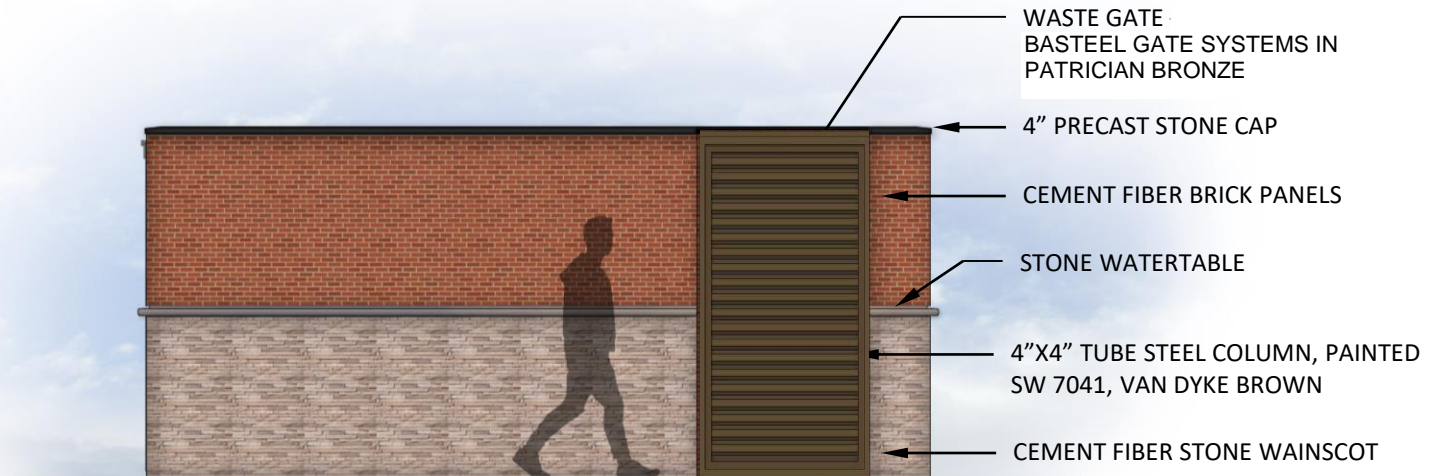
SIDE ELEVATION
