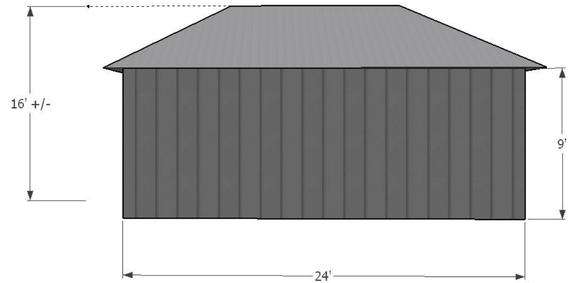
B GARAGE SIDE ELEVATION
