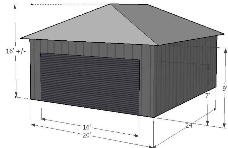
D GARAGE ISOMETRIC VIEW
