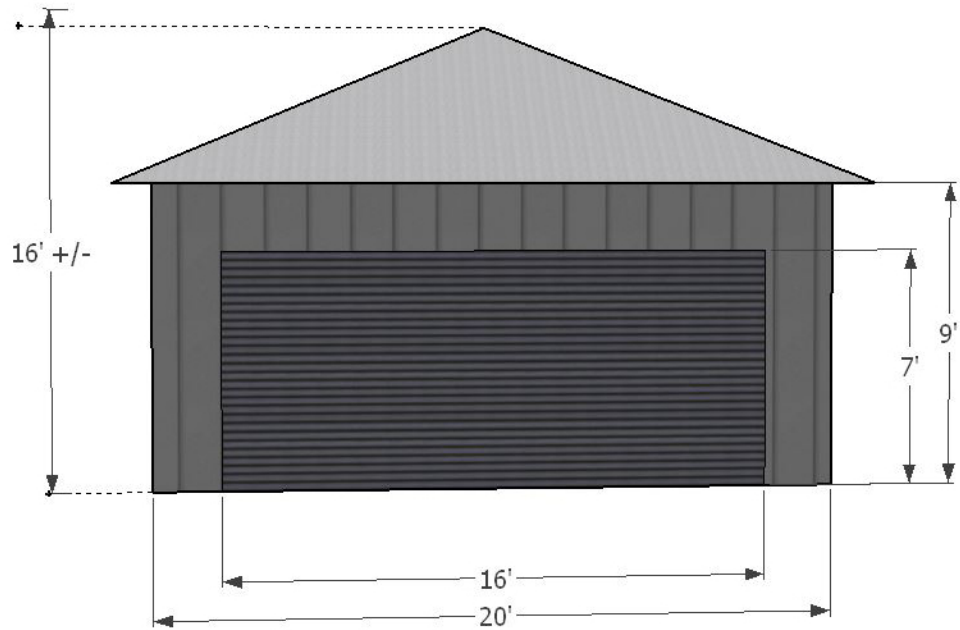
A GARAGE FRONT ELEVATION
