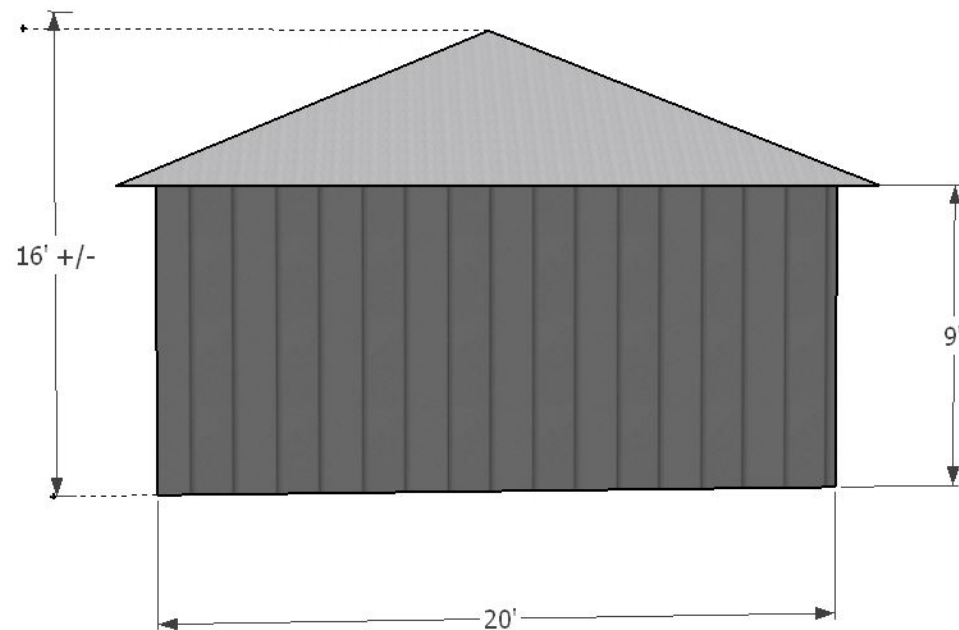
C GARAGE REAR ELEVATION
