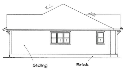
Left Side Elevation
