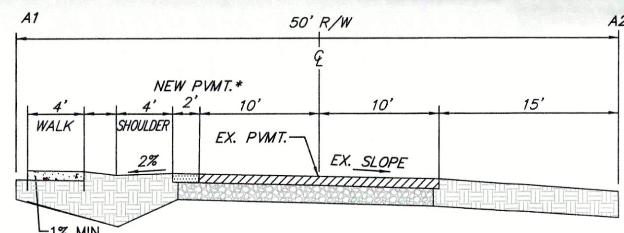
ROAD SECTION A NO SCALE *SEE PUBLIC WORKS NOTE #10
