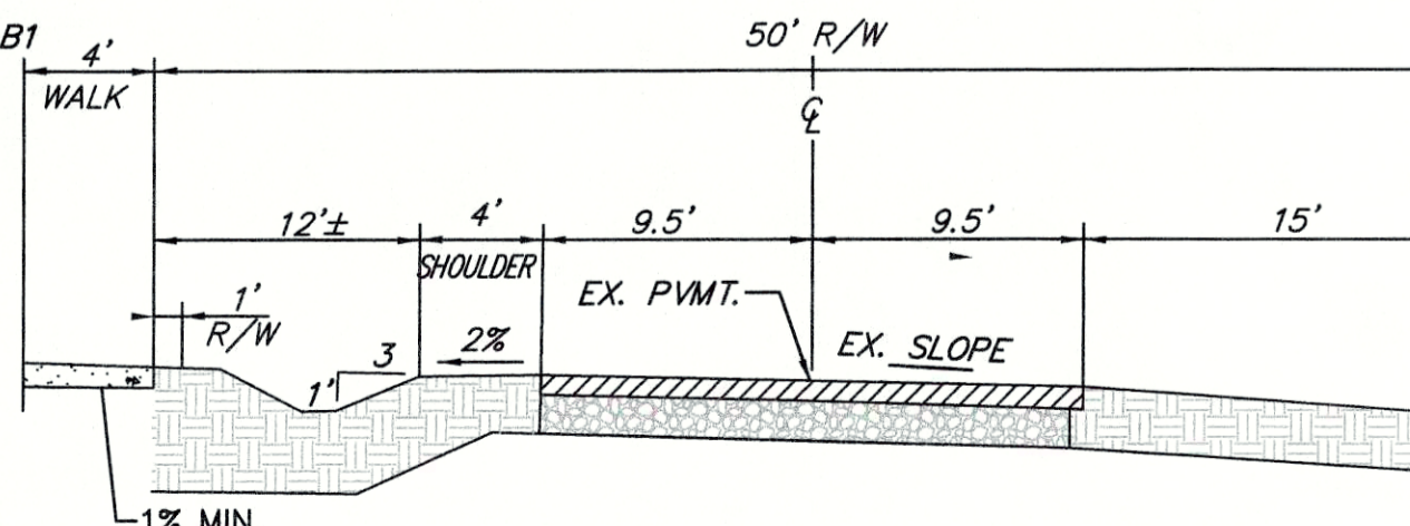
ROAD SECTION B NO SCALE
