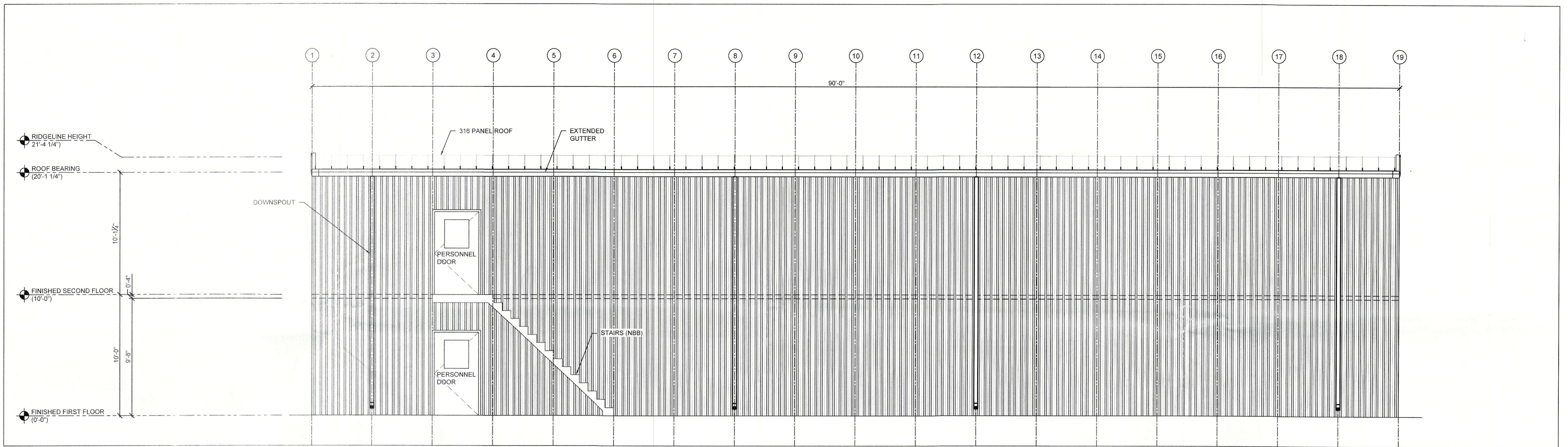
1 EXTERIOR ELEVATION (NORTH) 1/4" = 1'-0"
