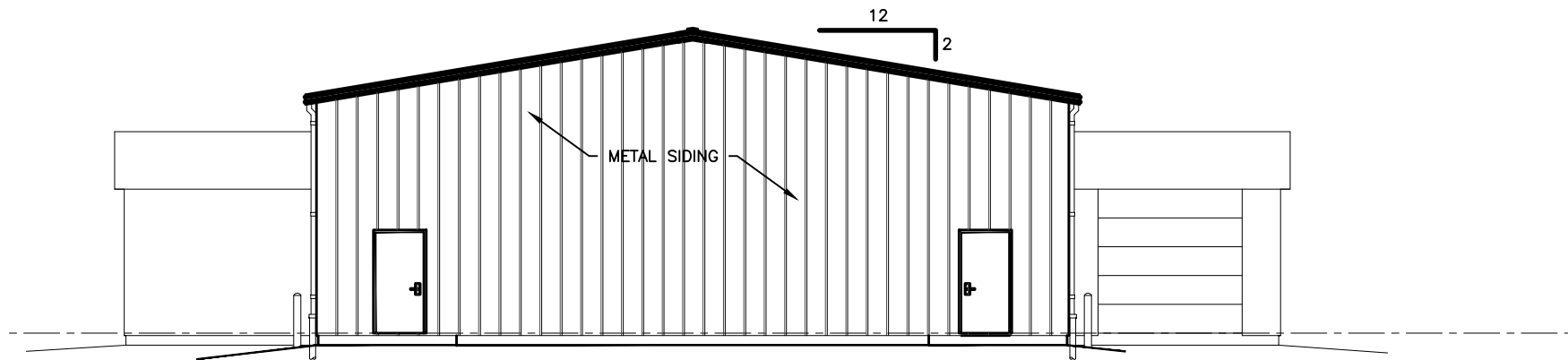
1 A1.1 PCR EXPANSION - SOUTH ELEVATION
