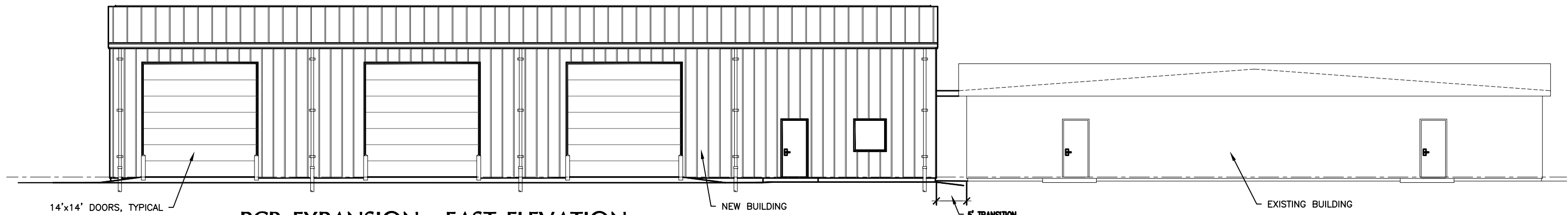
2 A1.1 PCR EXPANSION - EAST ELEVATION
