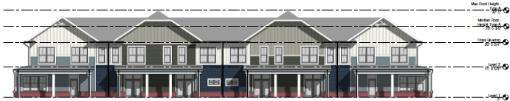
2 Elevation - Townhome - Type A - 6 Unit - Back - Schematic 002-101 1/8" = 1'-0"
