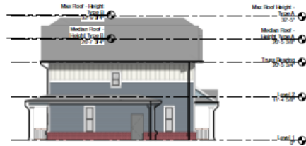
3 Elevation - Townhome - Type A - 6 Unit - Left - Schematic 002-101 1/8" = 1'-0"
