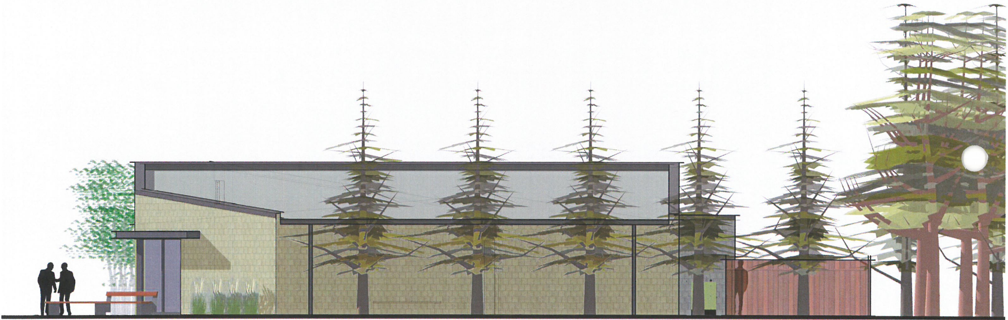
SOUTH ELEVATION
