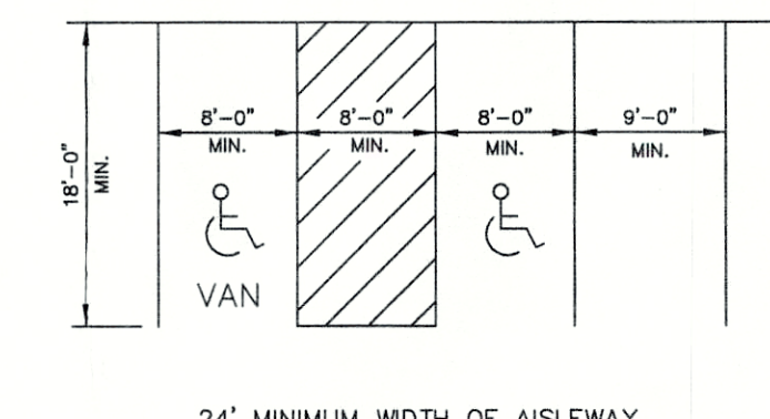
TYPICAL PARKING SPACE LAYOUT NO SCALE
