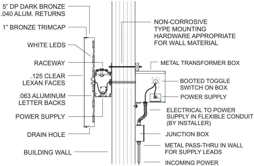
SECTION VIEW
