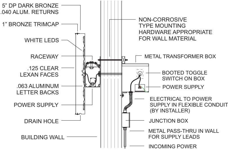
SECTION VIEW
