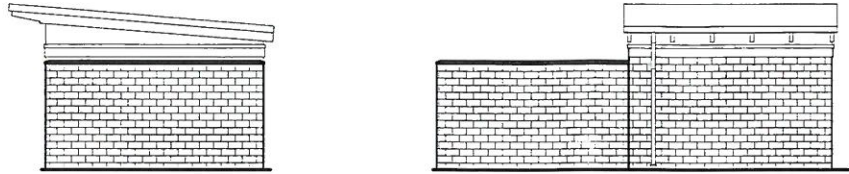
6 POOL EQUIPMENT BUILDING RIGHT AND REAR ELEVATION SCALE: 1/8" = 1'-0"
