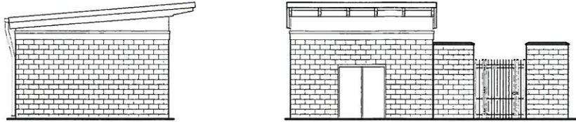
5 POOL EQUIPMENT BUILDING LEFT AND FRONT ELEVATIONS SCALE: 1/8" = 1'-0"
