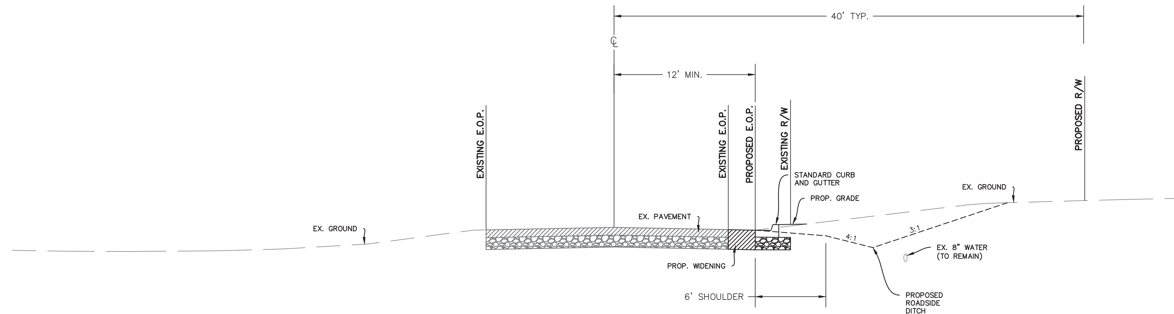
CEDAR CREEK ROAD TYPICAL SECTION NO SCALE
