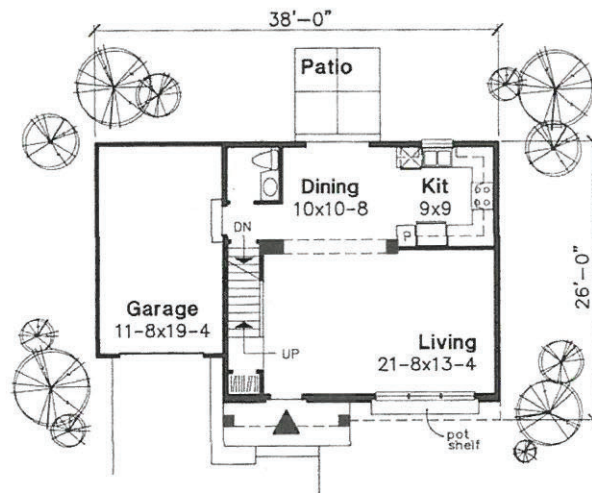
Plan Number 88160 | Order Code: TF00WEB | First Floor Plan
