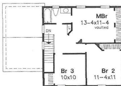
Plan Number 88160 | Order Code: TF00WEB | Second Floor Plan
