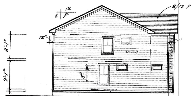
LEFT ELEVATION
